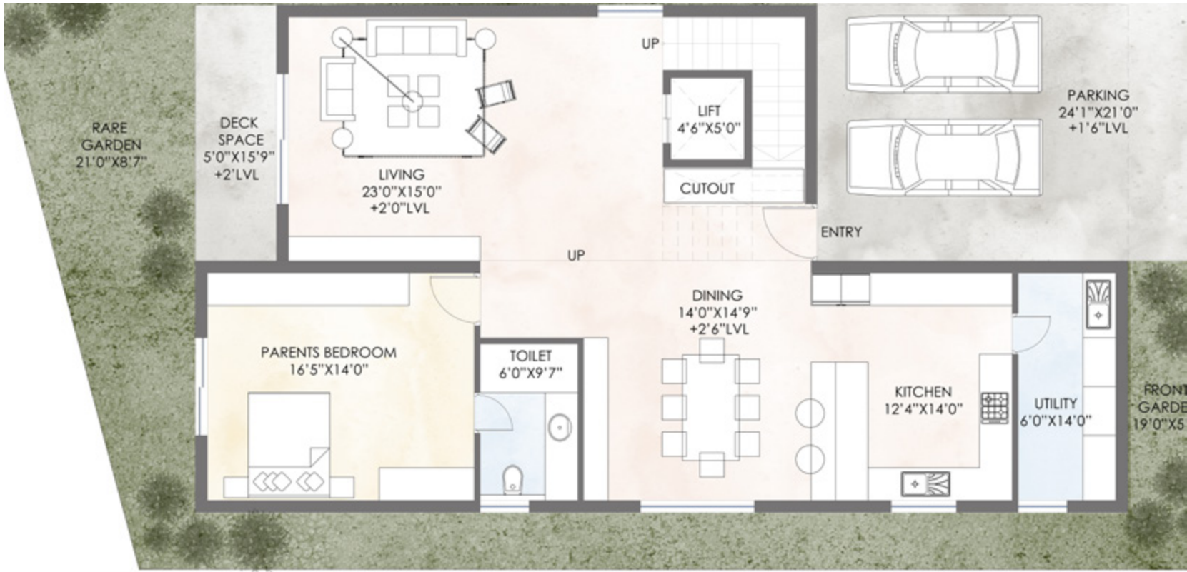
GROUND FLOOR
