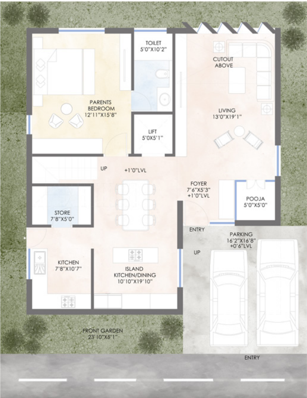
GROUND FLOOR
