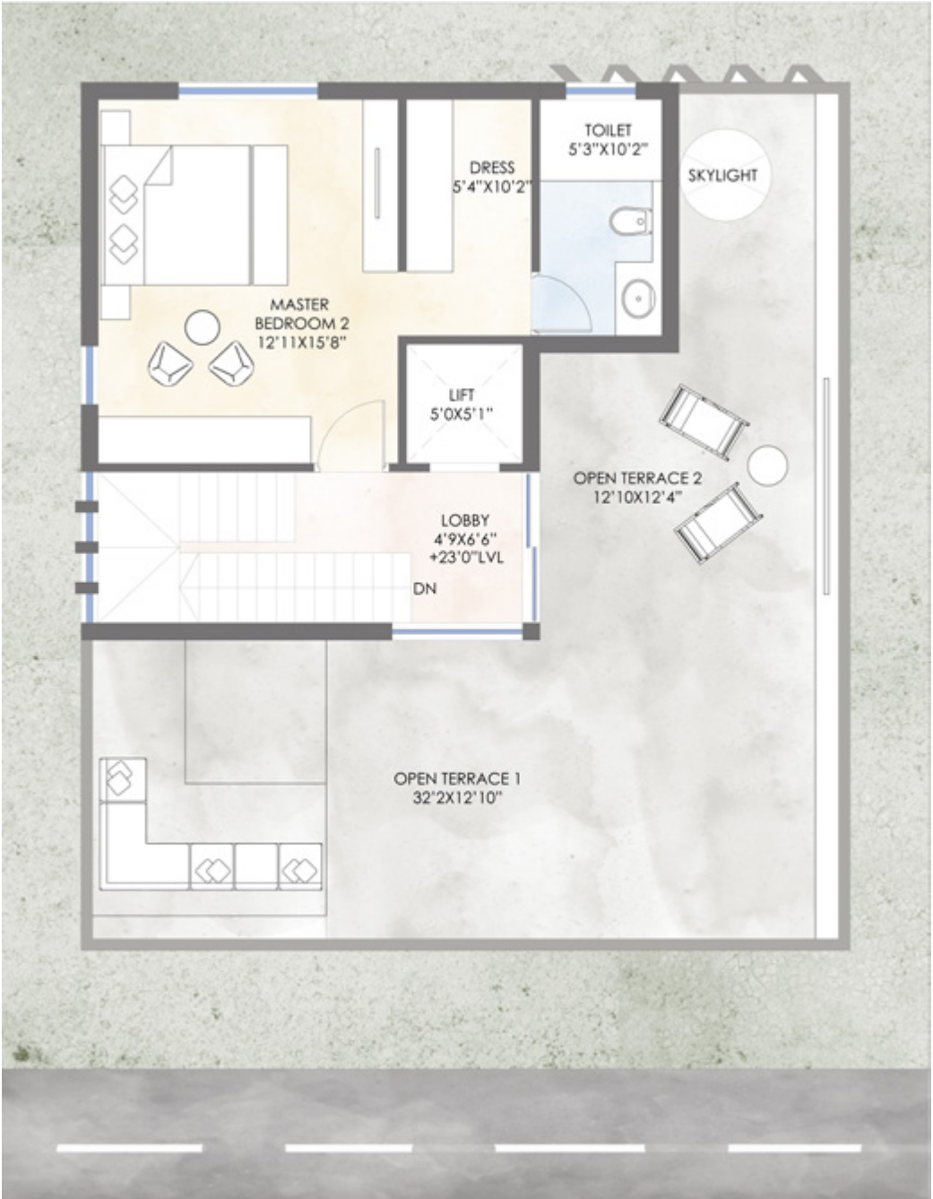
SECOND FLOOR
